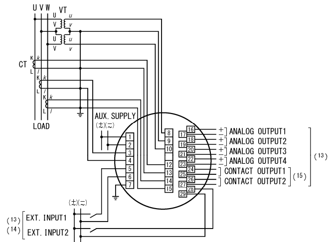
(4) 3φ3W (2VT, 3CT)
