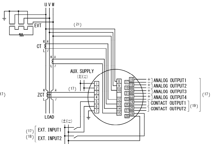
(4) 3φ3W (No grounding)
