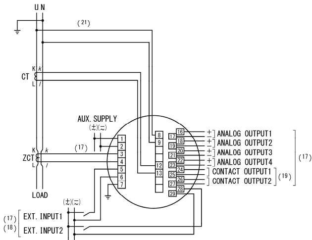
(1) 1φ2W (N-phase grounding)
