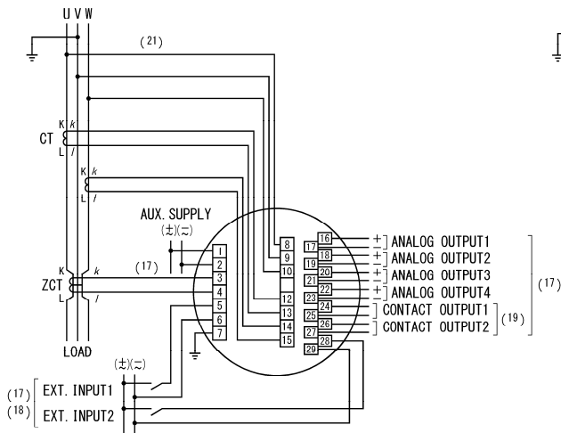
(3) 3φ3W (V-phase grounding)
