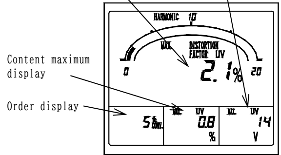
Voltage harmonic measurement maximum display.
