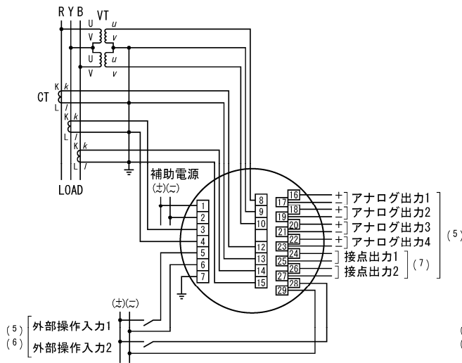
(1) 3φ3W (2VT, 3CT)
