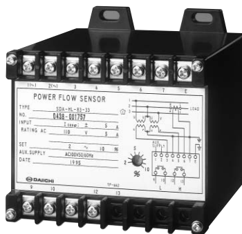
SDA-HL-83-33 (120 × 110 × 130mm/1.0kg)
