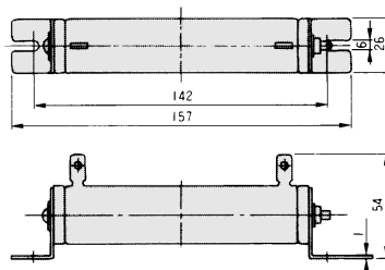
DC110V用倍率器 (RWH60G)
