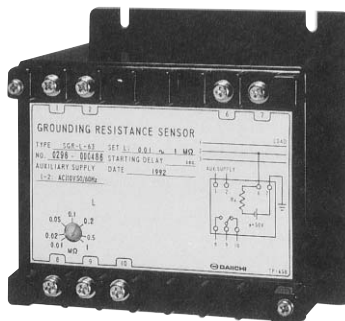
SGR-L-63 (120 × 110 × 112mm/1.0kg)
