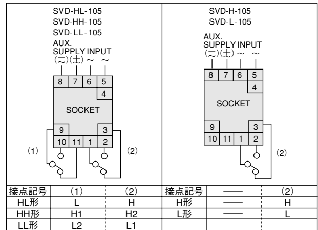
SVD-HL-105 (80×50×131mm/320g)
